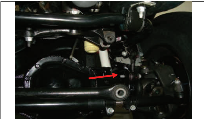
05-10 Disconnect lower sway bar mounting hardware
