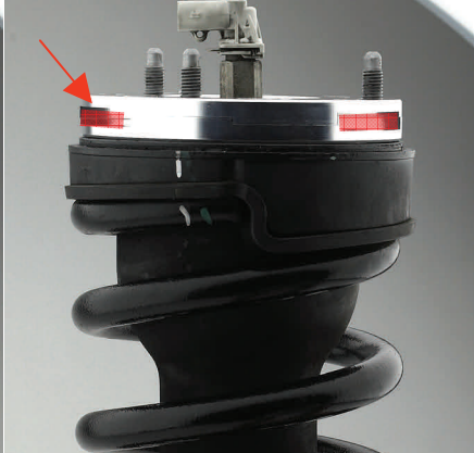
Figure 5 A-B = 1.25" at the wheel
